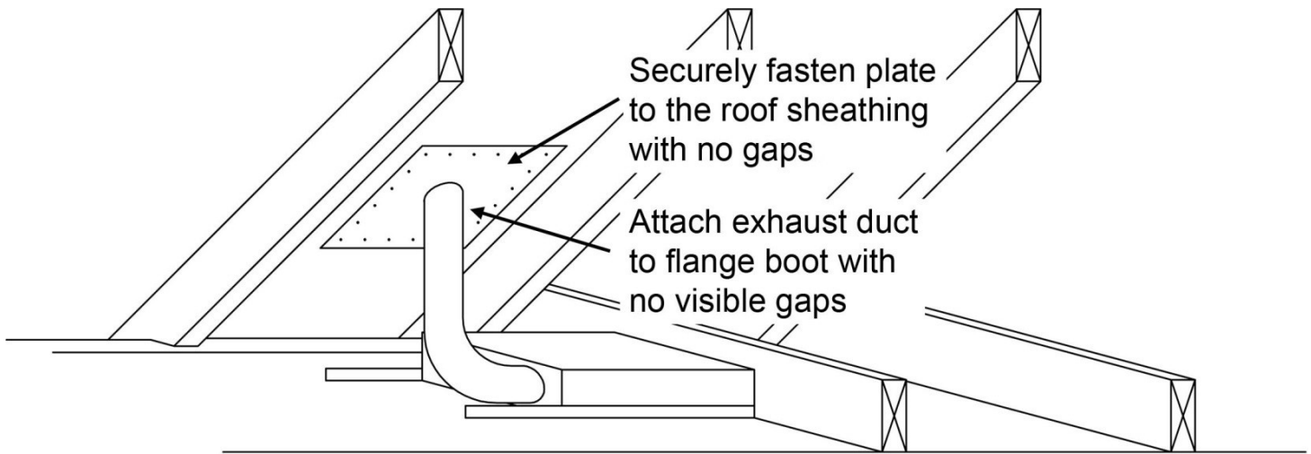
Illustration AT 1.6—Exhaust boot connected to sheathing
