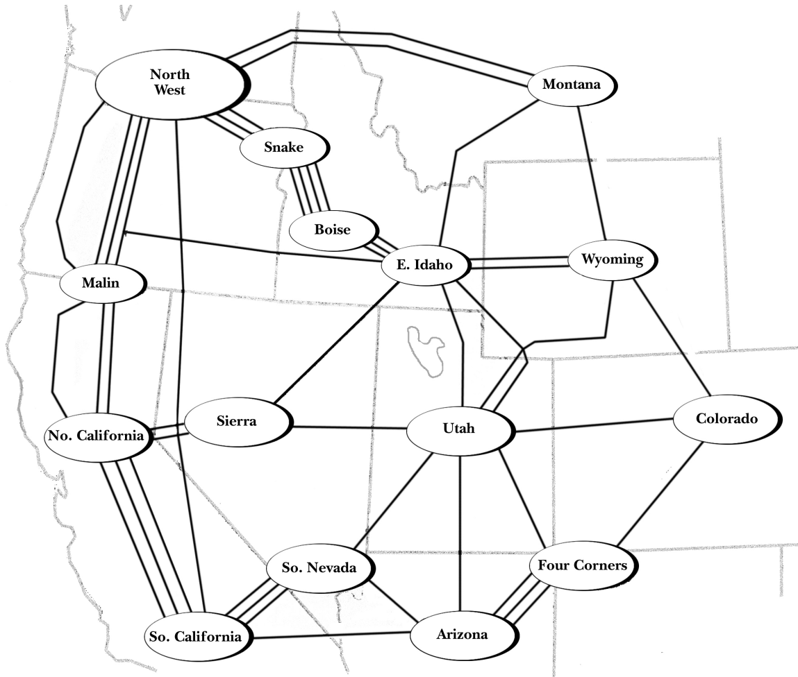
Figure 1—Simplified Map of Interconnected Western Power System
