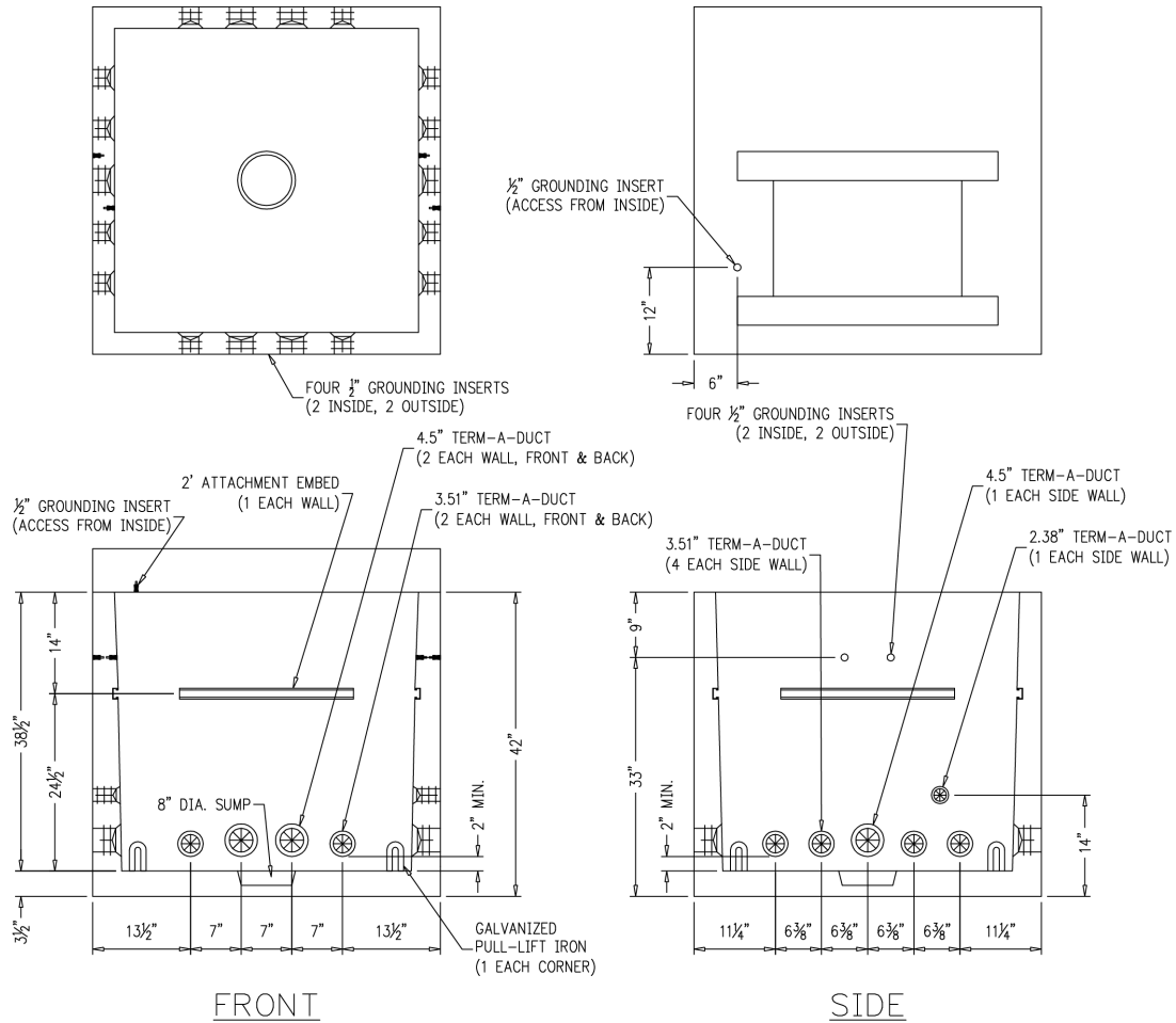
Figure 2 — 4' x 4' Vault Layout
