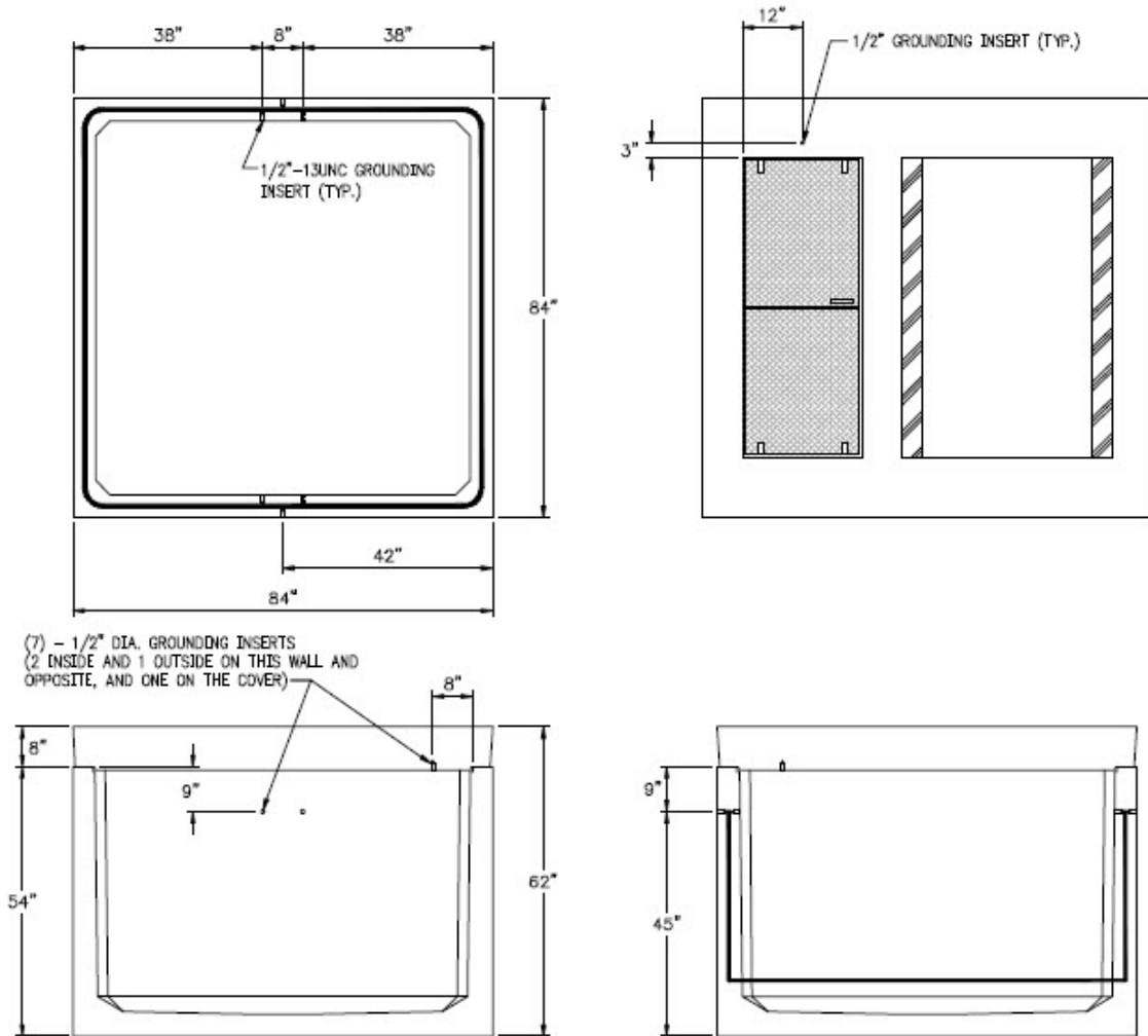
Figure 4—Ground Grid Layout for 7' × 7' (84" × 84") Shallow Vault
